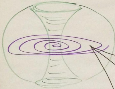
Milky Way
