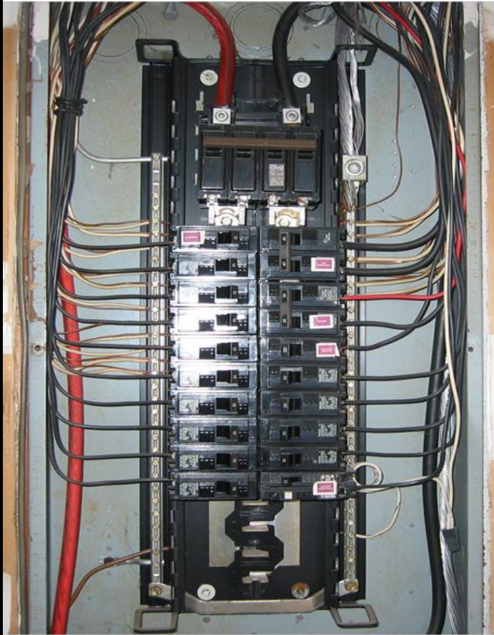
Breaker Box
